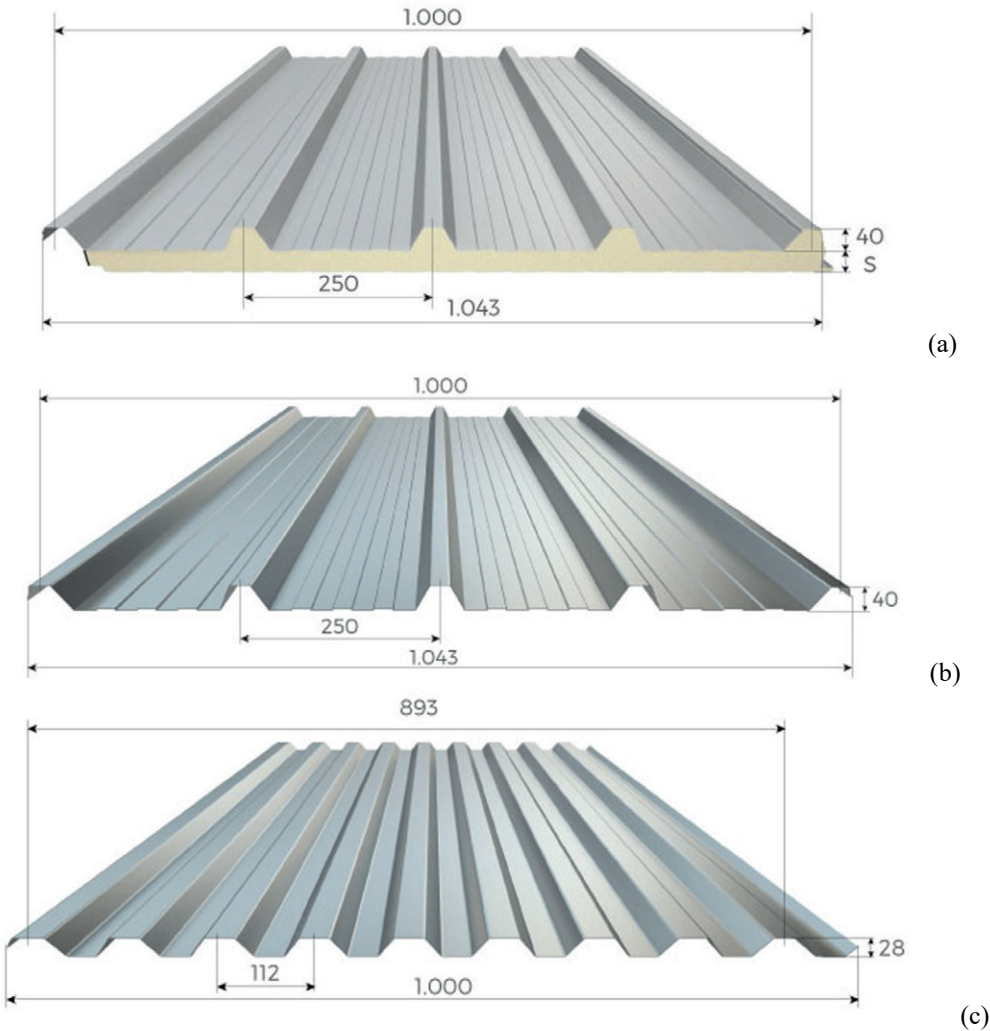
Figure 20 – (a) Sandwich panel; (b) Steel ribbed sheet; (c) Aluminium ribbed sheet
